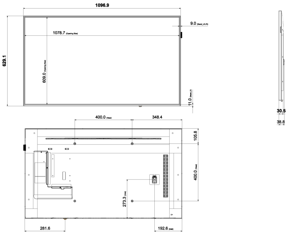
DCH/PMH 49inch Mechanical Drawing_170126
